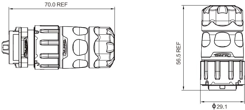
Cable Connector
