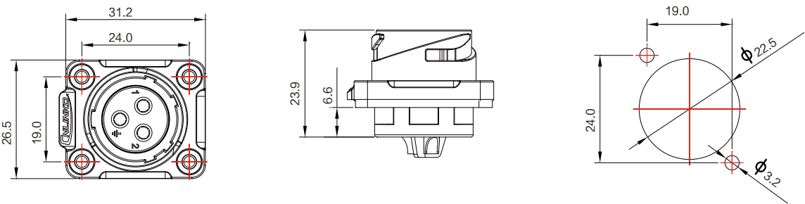
Flange Mounting
